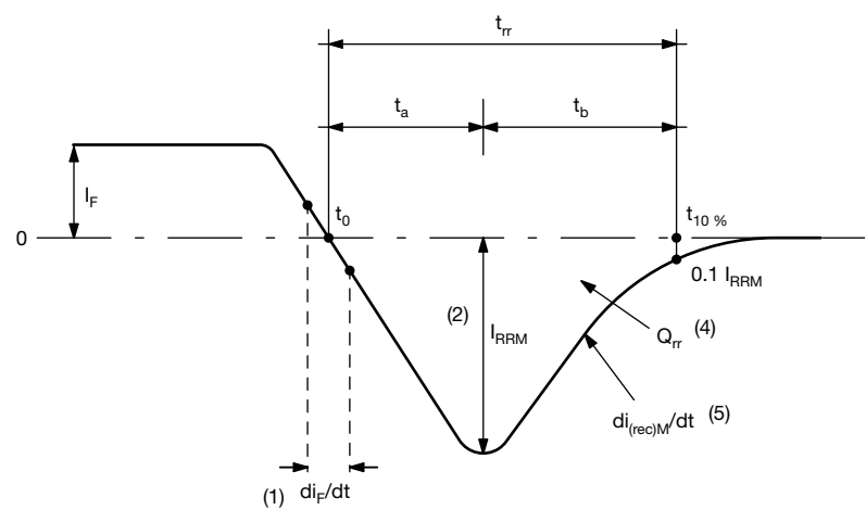
Reverse Recovery Waveform and Definitions
