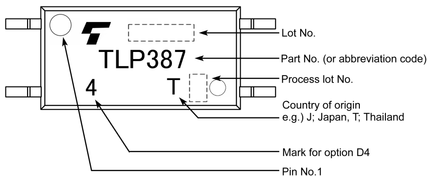
Fig. 15.3 Marking Example (Note 1)
