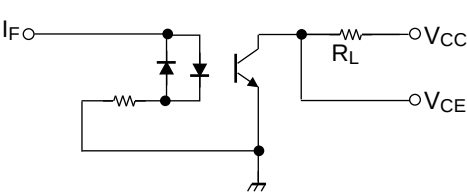
(Fig. 2): Switching time test circuit
