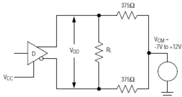
Figure 2. Driver V_{OD} with Varying Common-Mode Voltage
