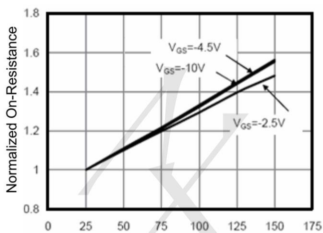
Figure 8 Drain-Source On-Resistance
