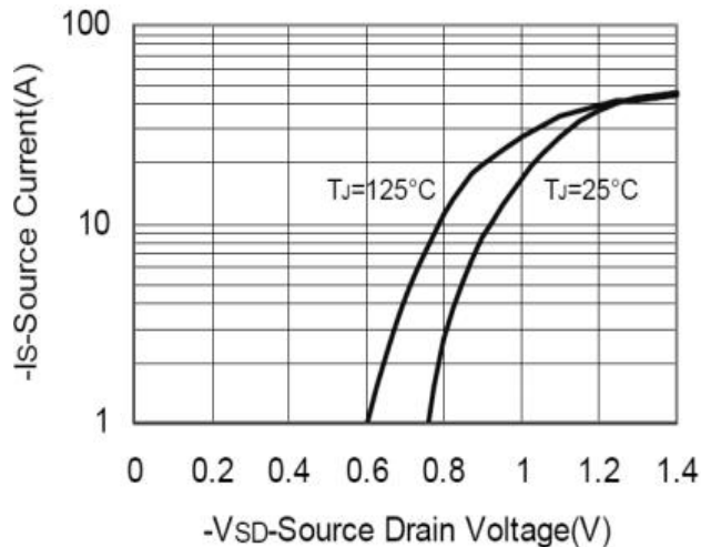
Figure 8: Diode Characteristics
