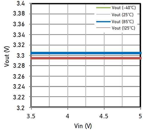
Line Regulation V_{OUT} vs. V_{IN} C_{OUT} = C_{IN} = 1\mu F, I_{OUT} = 30mA
