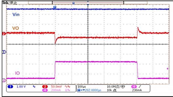
Load-Transient Response
