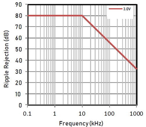
Ripple Rejection vs. Frequency I_{OUT} = 30mA, C_{OUT} = 1\mu F
