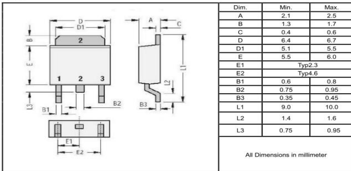
TO-252
