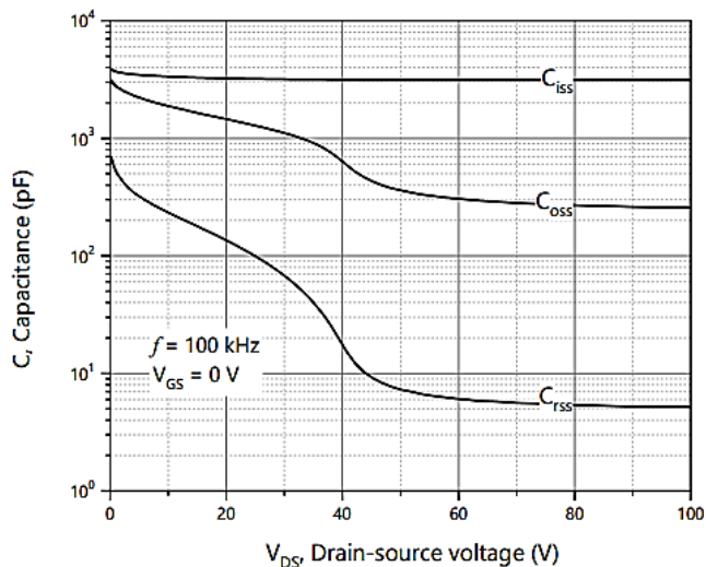
Figure 3. Typ. capacitances
