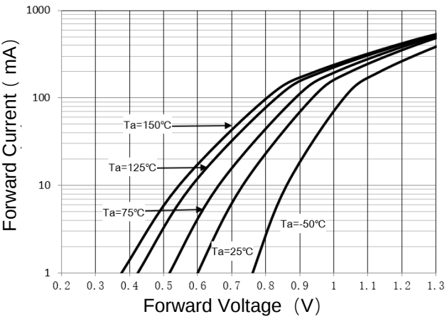
Fig 2. V_F characteristics
