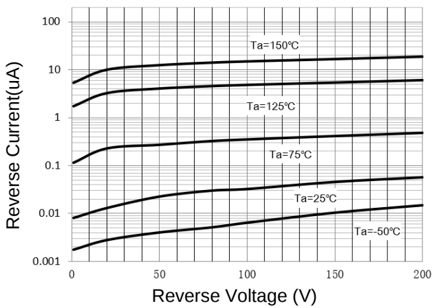
Fig 1. V_R characteristics
