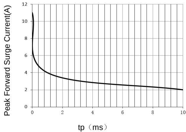
Fig 3. IFSM Curve
