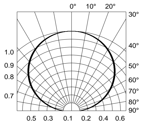
Fig.6-Radiation Diagram Ta=25°C
