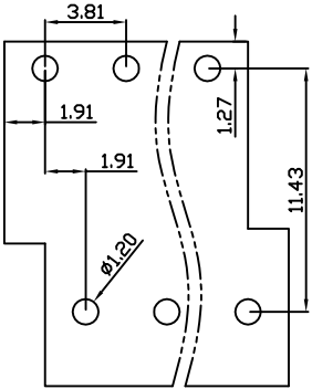
PCB Layout
