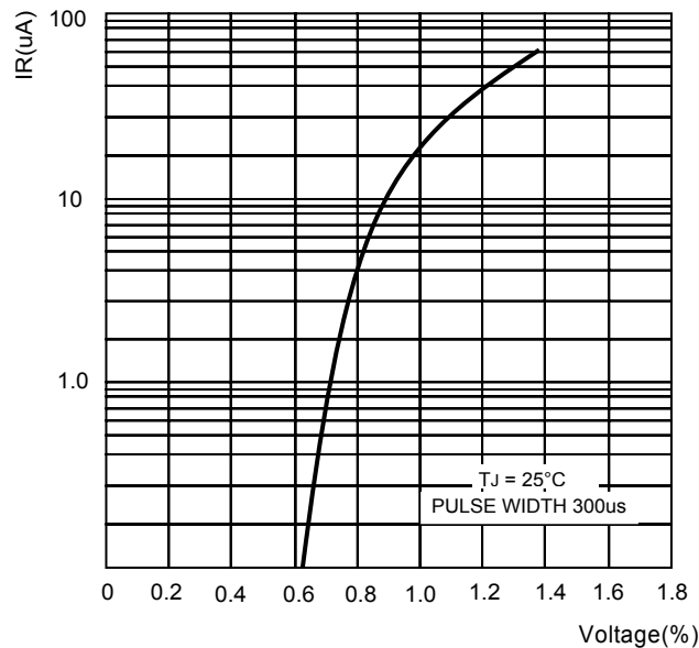
FIG.4-TYPICAL REVERSE CHARACTERISTICS
