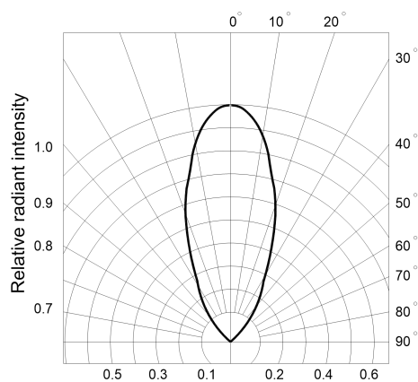
Fig.6 Radiation diagram
