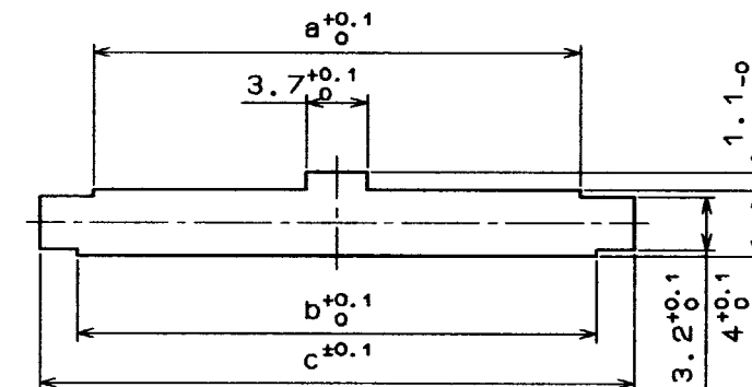
< PANEL CUTOUT >
