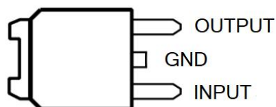
TO252 (TOP VIEW)
