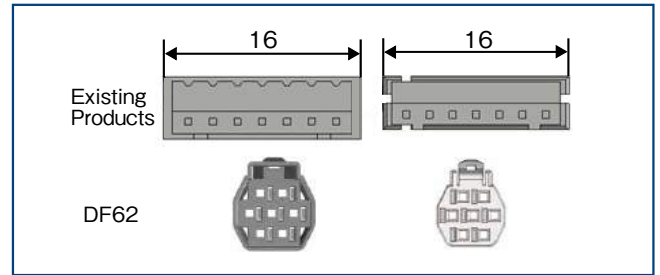
Compact shape due to 2 \times 2 grid layout of pins (Both are 7 contacts with 3A current rating)
