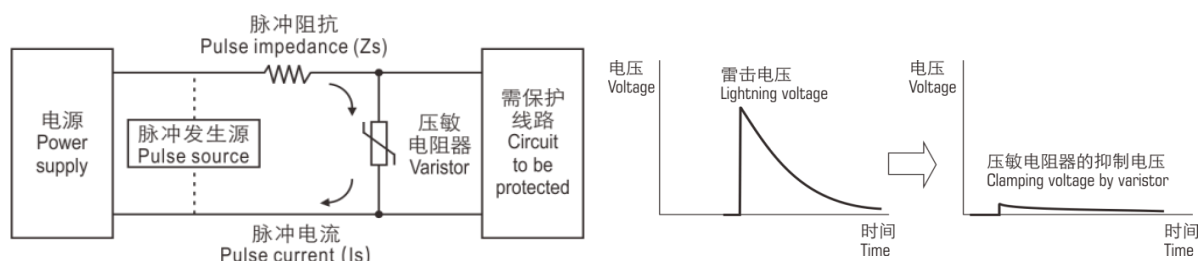
壓敏電阻器對脈衝的吸收 PULSE ABSORPTION BY VARISTOR
