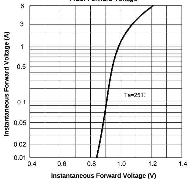
FIG3: Forward Voltage
