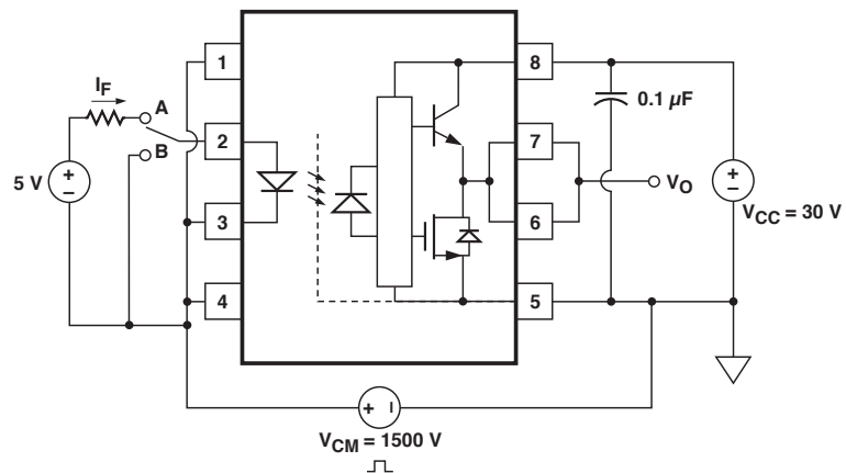
Figure 24. CMR test circuit and waveforms.
