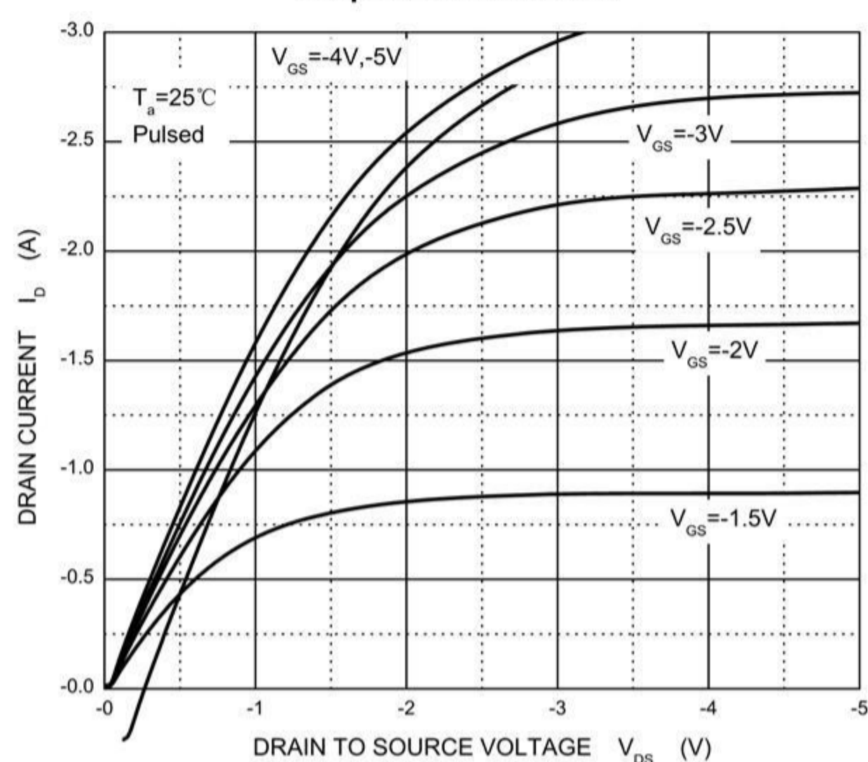
Output Characteristics
