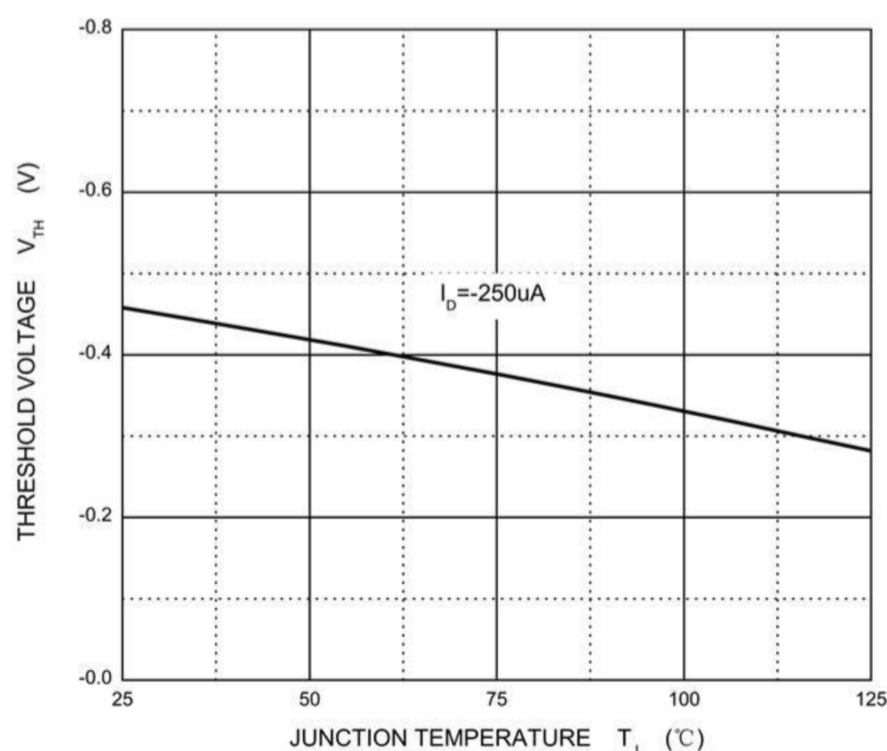
Threshold Voltage
