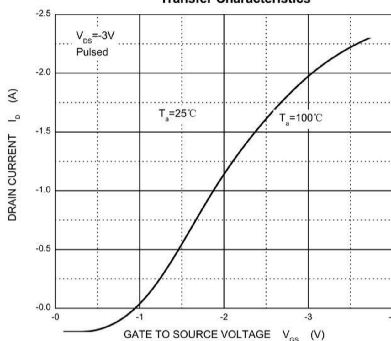
Transfer Characteristics
