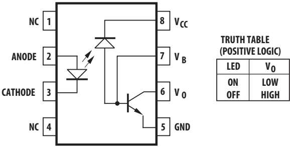
Truth Table (Positive Logic)
