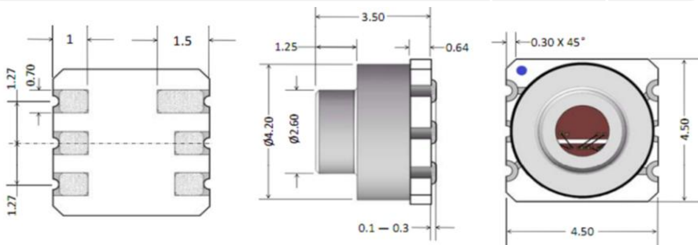
Figure2. Package Outline
