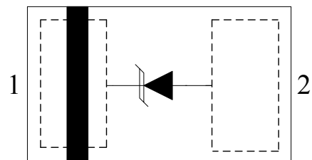
DFN1006-2L (Top View)
