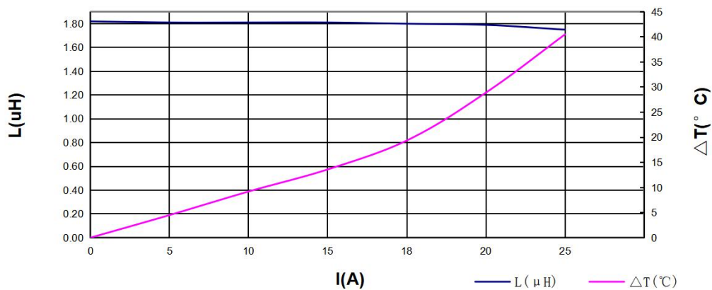
CURRENT CHARACTERISTIC
