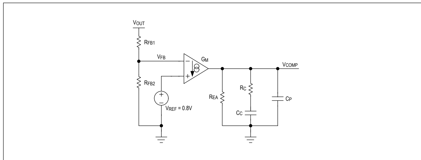
Figure 2. Compensation Network
