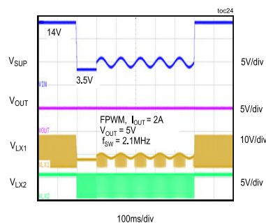
COLD CRANK
