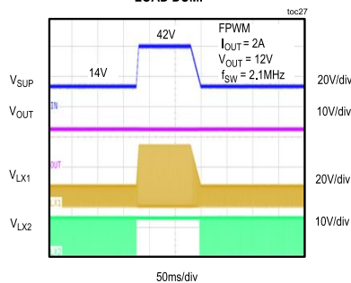
LOAD DUMP
