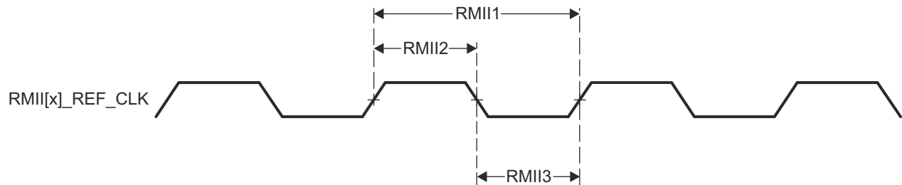
Figure 7-10. CPSW3G RMII[x]_REF_CLK Timing Requirements – RMII Mode
