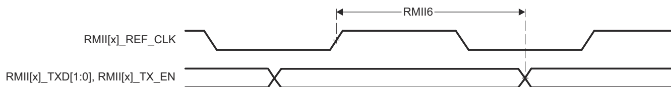
Figure 7-12. RMII[x]_TXD[1:0], and RMII[x]_TX_EN Switching Characteristics – RMII Mode
