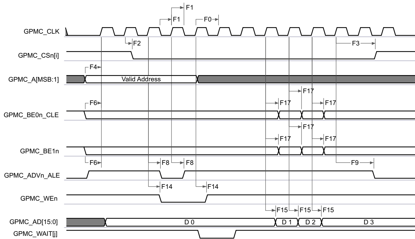
Figure 7-26. GPMC and NOR Flash — Synchronous Burst Read — 4x16-bit (GPMCCLKDIVIDER = 0)
