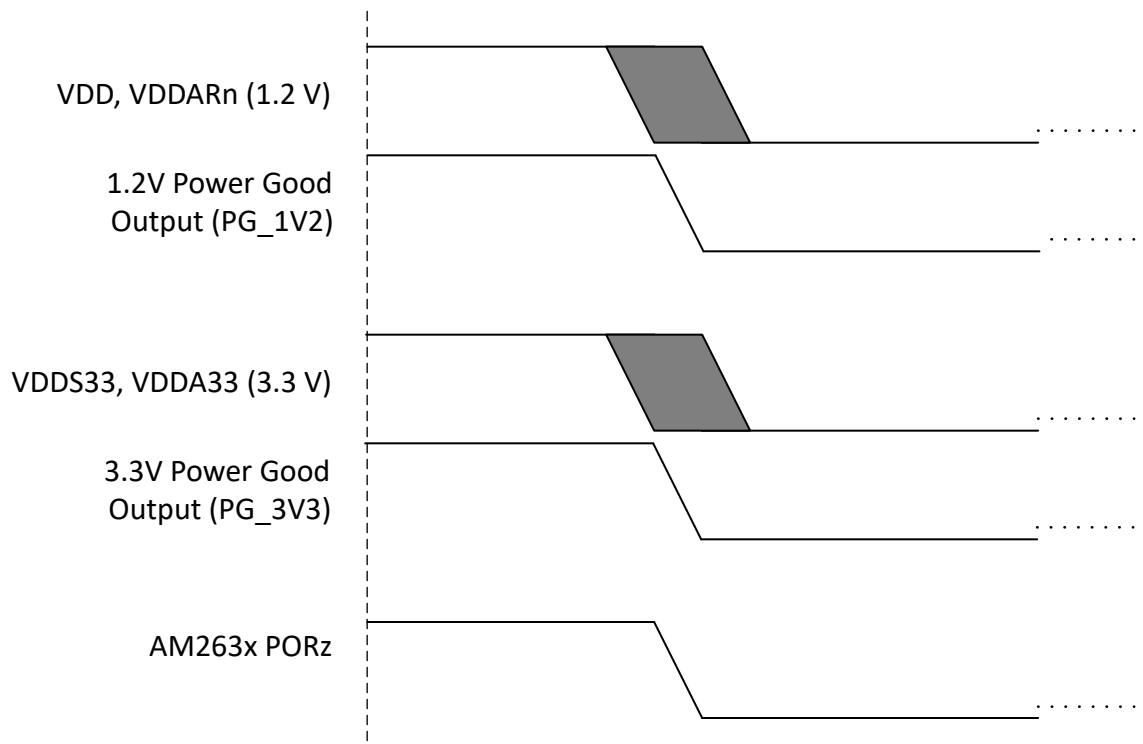
Figure 7-2. Power-Down Sequencing
