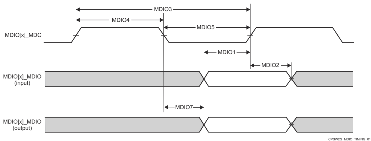
Figure 7-9. CPSW3G MDIO Timing Requirements and Switching Characteristics
