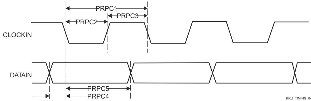
Figure 7-52. PRU-ICSS PRU Parallel Capture Timing Requirements – Falling Edge Mode
