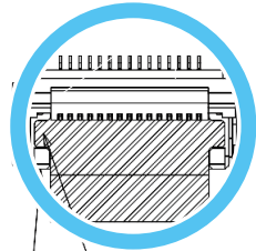
FPC/FFC Positioning Tab FPC/FFC Positioning Guide
