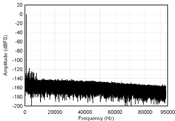
图 9-10. Noise Performance FFT Plots with Sinc4 Filter for G = 0.2 \text{ V/V}
