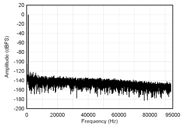
图 9-11. Noise Performance FFT Plots with Sinc4 Filter for G = 1 \text{ V/V}
