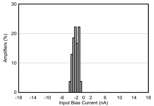
图 7-8. Typical Distribution of Input Bias Current
