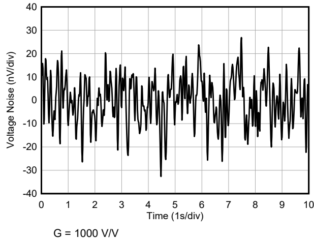
图 7-29. 0.1-Hz to 10-Hz RTI Voltage Noise
