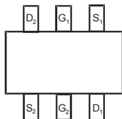
Top View Internal Schematic
