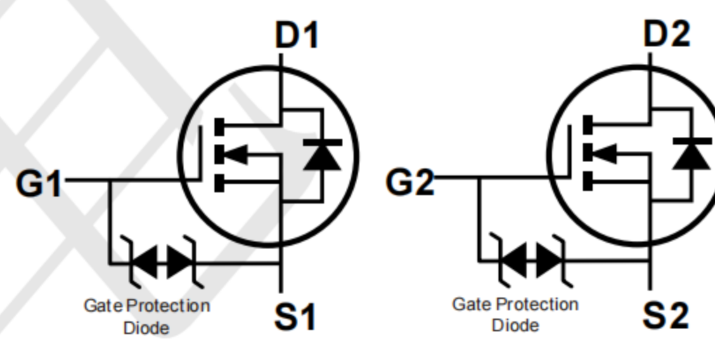
Equivalent Circuit
