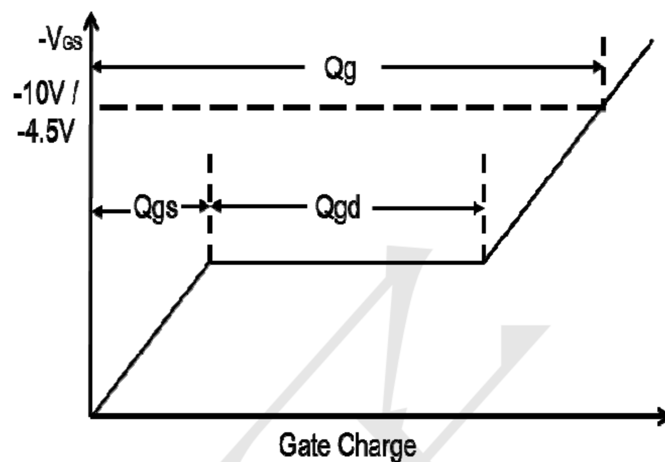
Figure 8. Gate Charge Waveform
