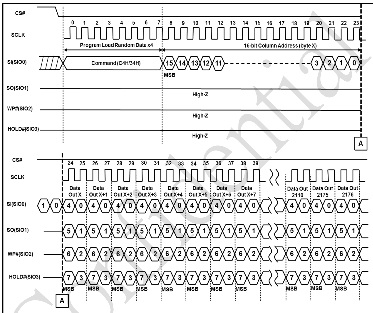
Program Load Random Data x4 (C4H/34H) Sequence Diagram
