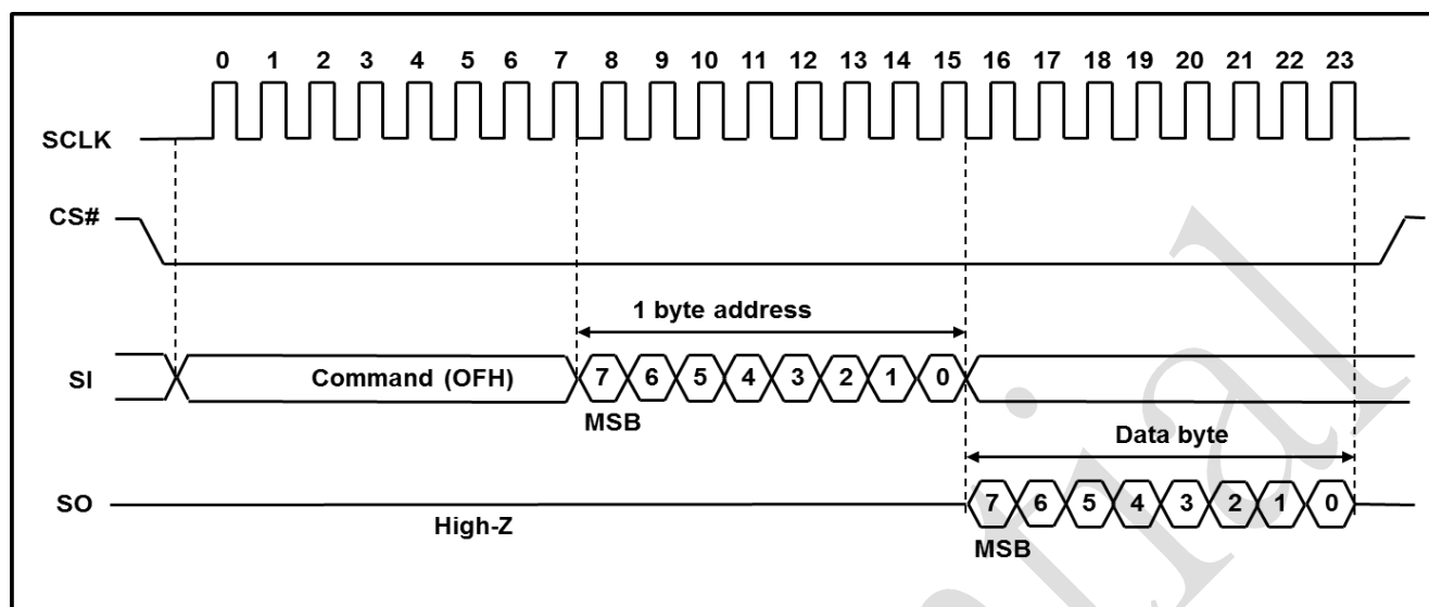
Get Feature (0FH) Sequence Diagram
