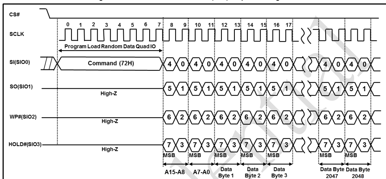
Program Load Random Data Quad IO (72H) Sequence Diagram
