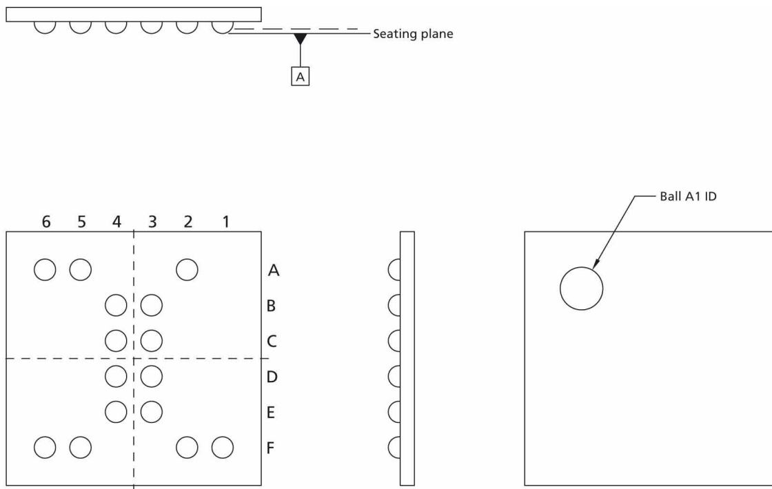
Figure 11: 15-Ball XFWLBGA
