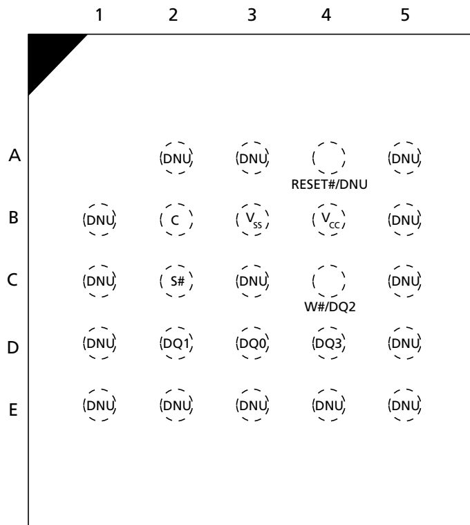
Figure 4: 24-Ball T-BGA, 5 × 5 (Balls Down)
