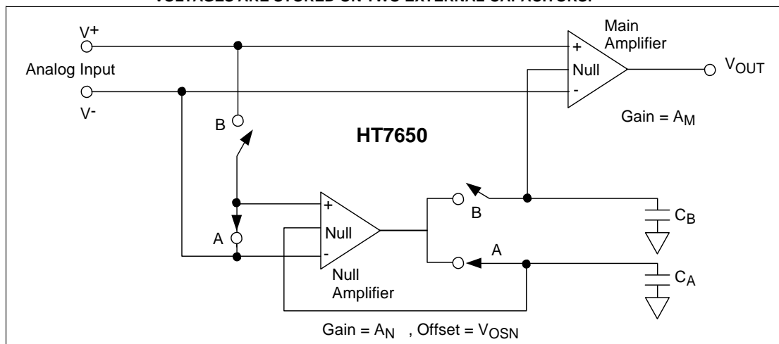
FIGURE 3-2: NULLING CAPACITOR CONNECTION
