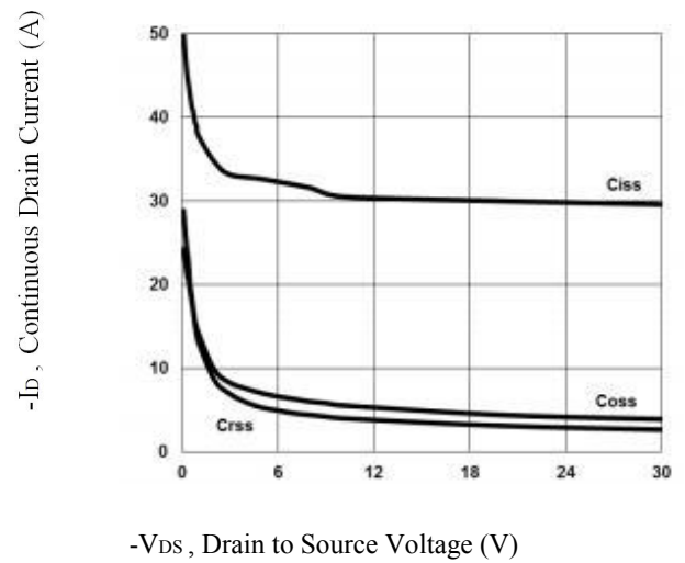
Fig. 6 Capacitance Characteristics
