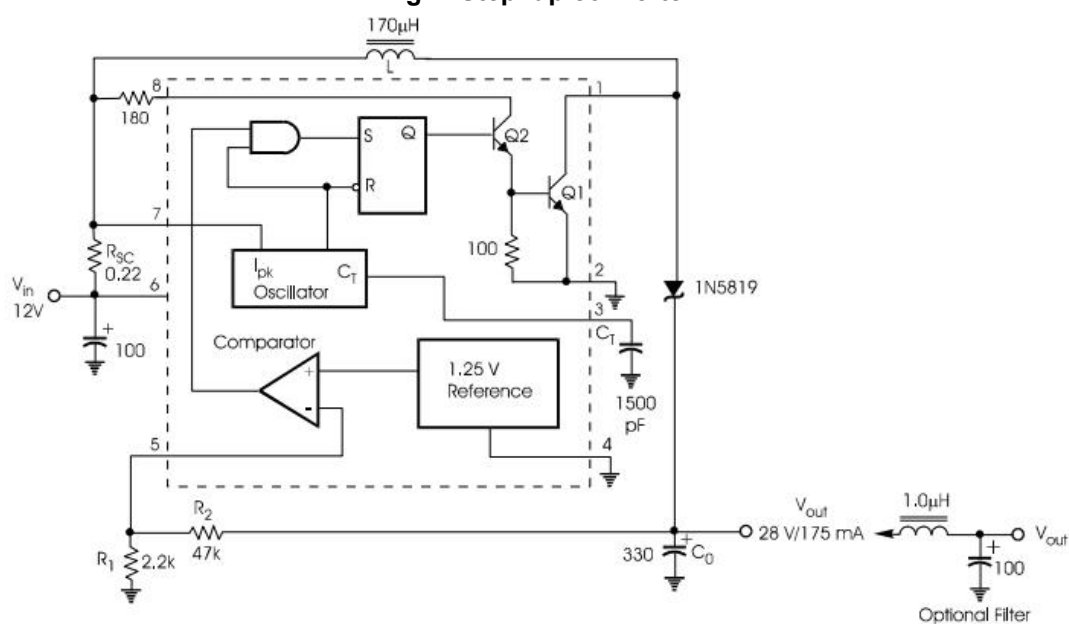
Fig.1. Step-up converter
