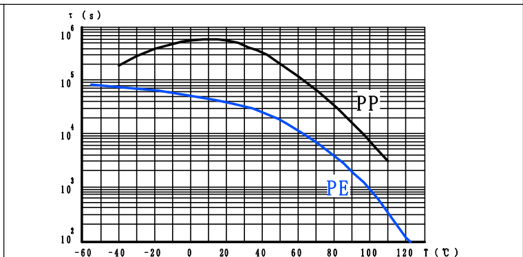
绝缘电阻与温度的关系(CR value) IR vs. Temperature
