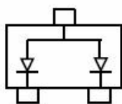
BAT54AW MARKING:L42
