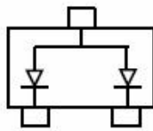
BAT54AW MARKING:L42
