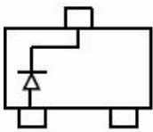
BAT54W MARKING:L4
