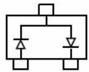
BAT54SW MARKING:L44
