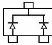
BAT54CW MARKING:L43
