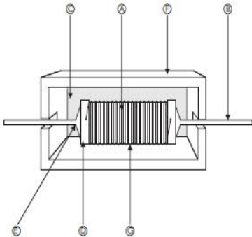
WIRE WOUND CEMENT TYPE 绕线水泥电阻
