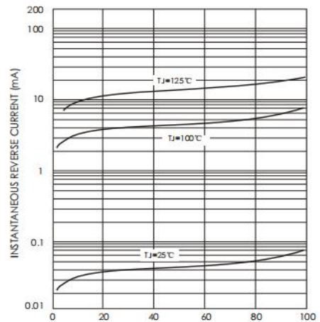
FIG.4-TYPICAL REVERSE CHARACTERISTICS
