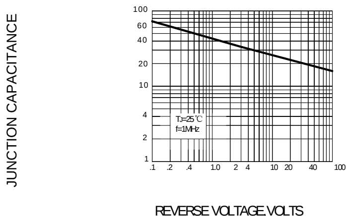
FIG.5-TYPICAL JUNCTION CAPACITANCE
