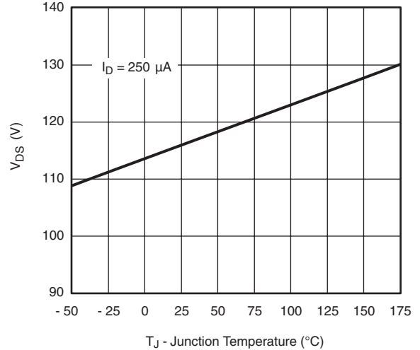
T J - Drain-Source Breakdown vs. Junction-Temperature
