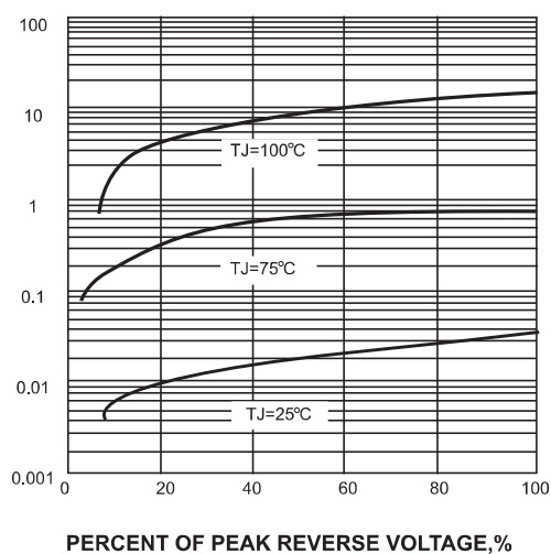
FIG. 4-TYPICAL REVERSE CHARACTERISTICS
