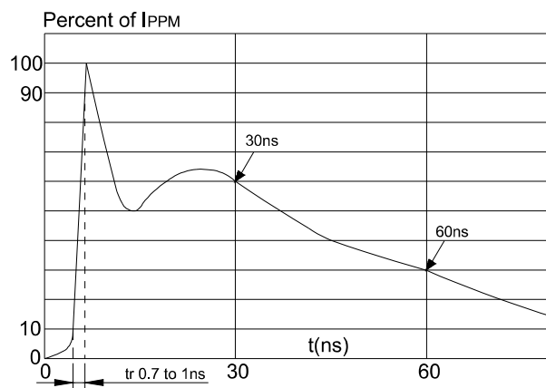
FIG.4: ESD clamping
