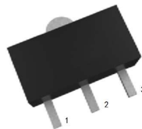
1: OUT 2: GND 3: IN
