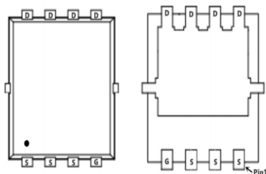
DFN5*6-8L
