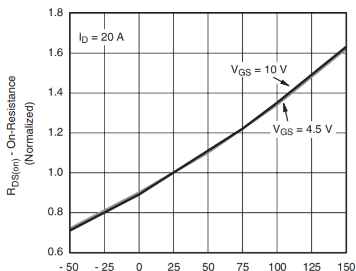
On-Resistance vs. Junction Temperature
