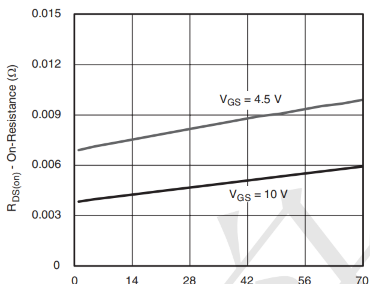
On-Resistance vs. Drain Current
