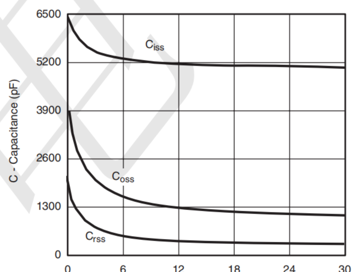
Capacitance
