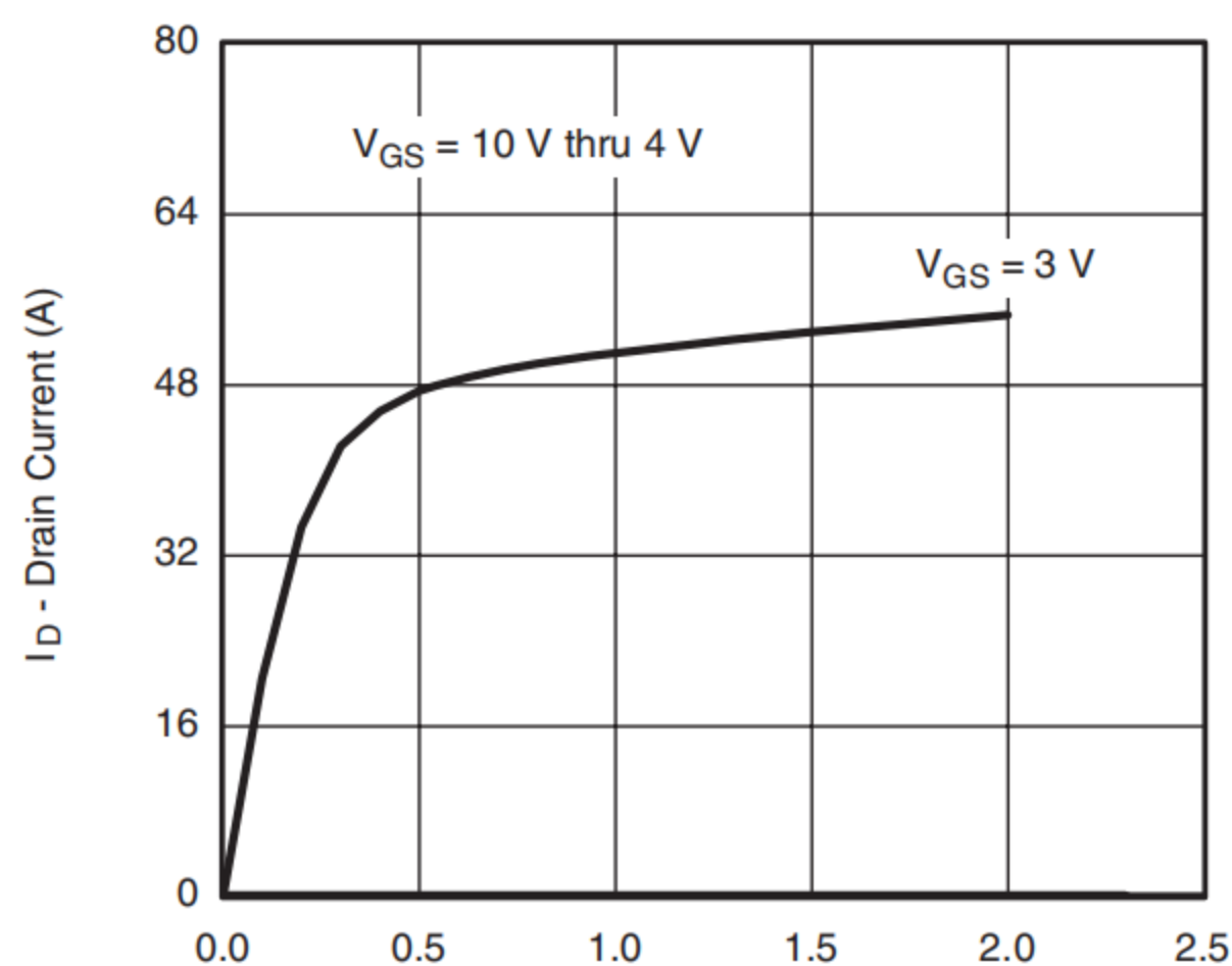
Output Characteristics
