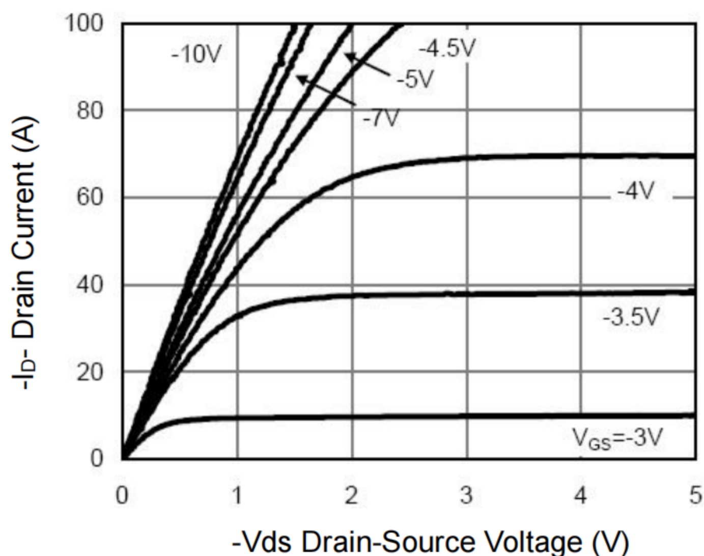
Figure 1 Output Characteristics
