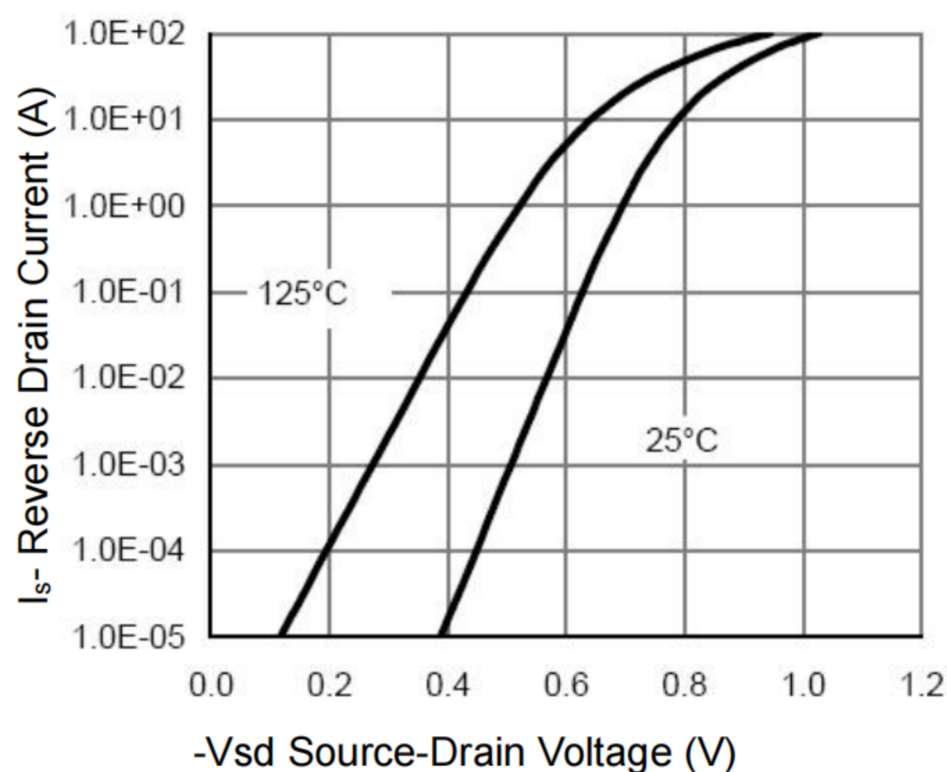
Figure 6 Source- Drain Diode Forward
