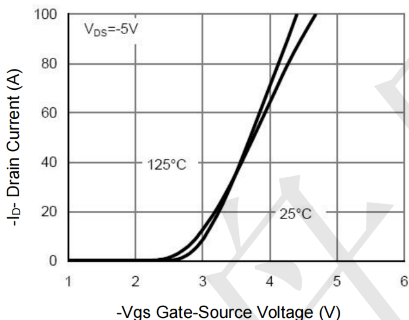
Figure 2 Transfer Characteristics
