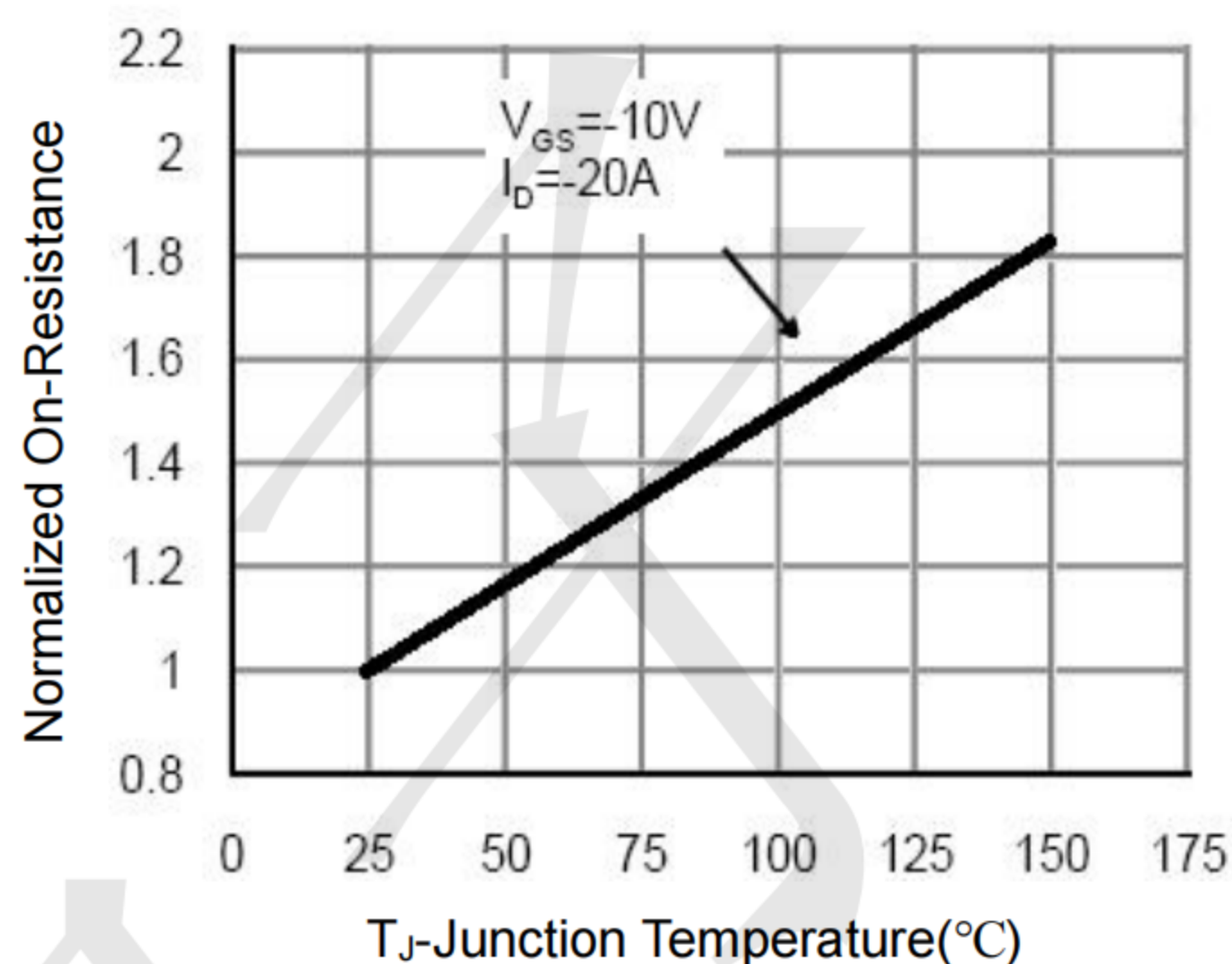
Figure 4 Rdson-Junction Temperature
