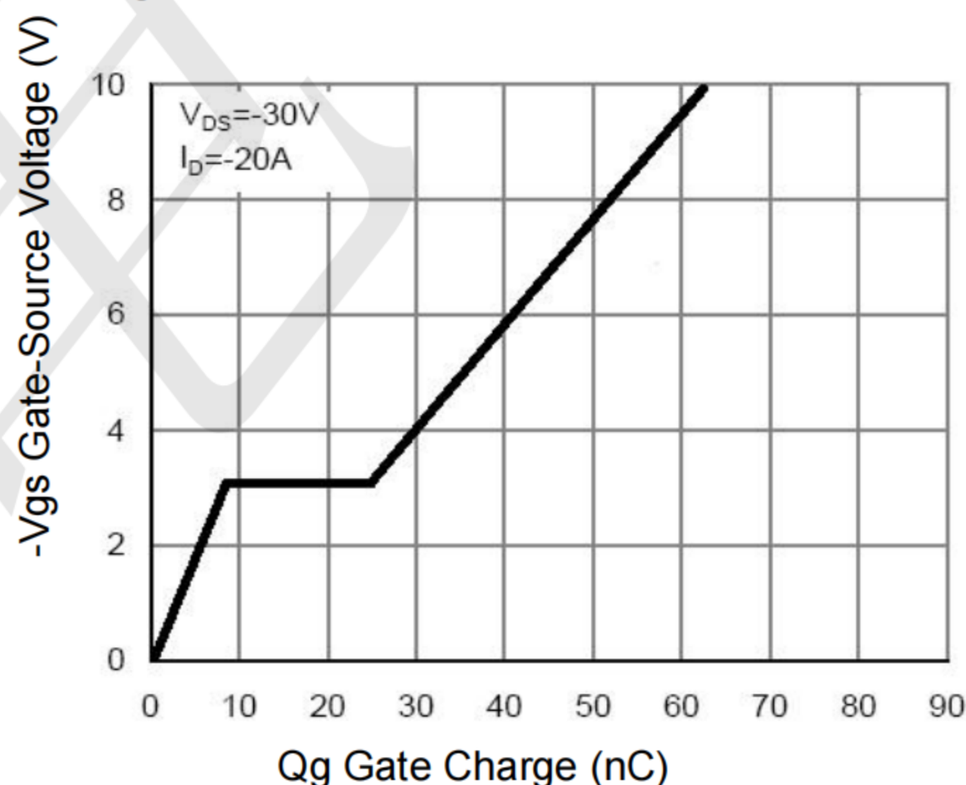
Figure 5 Gate Charge
