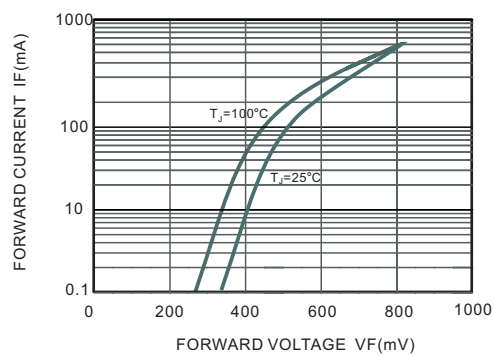
Fig.3 Forward Characteristics
